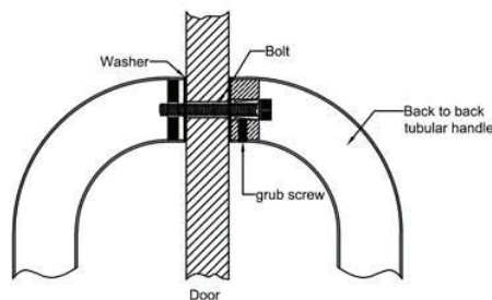
Back to back standard fixing
